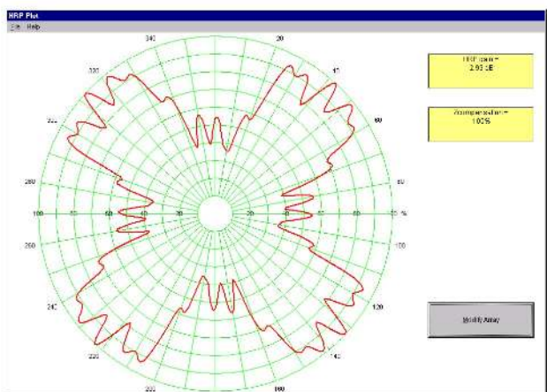
Skew Fire 4 Panels Radius 1465mm @ 680MHz
