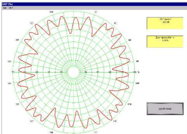
Skew Fire 4 panels Radius 1465mm @600MHz
