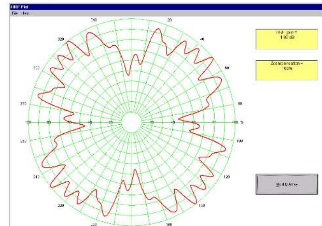
Skew Fire 4 panels Radius 1465mm @620MHz
