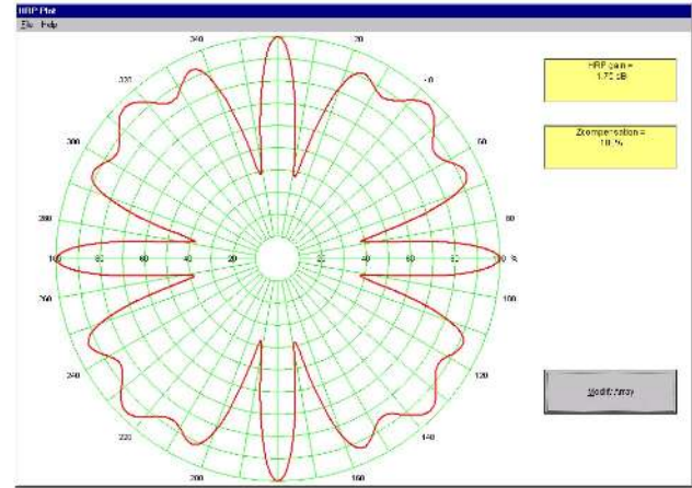
Radial Fire Radius 750mm @600MHz
