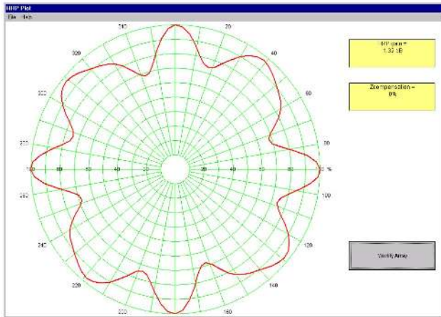
Radial Fire Radius 350 Offset 120 @ 600MHz
