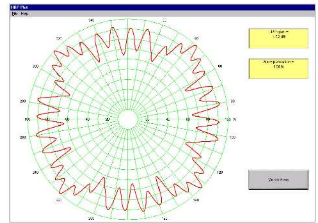
Skew Fire 4 Panels Radius 1465mm @ 740MHz
