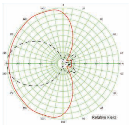
HRP & VRP Mounted to 100mm Dia Pole on 2800mm Face Structure
