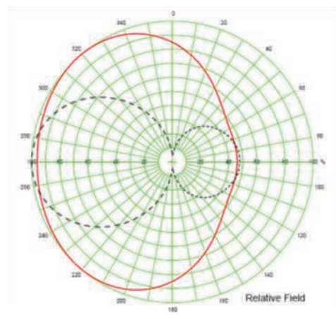
HRP & VRP Mounted to 100mm Dia Pole in Free Space
