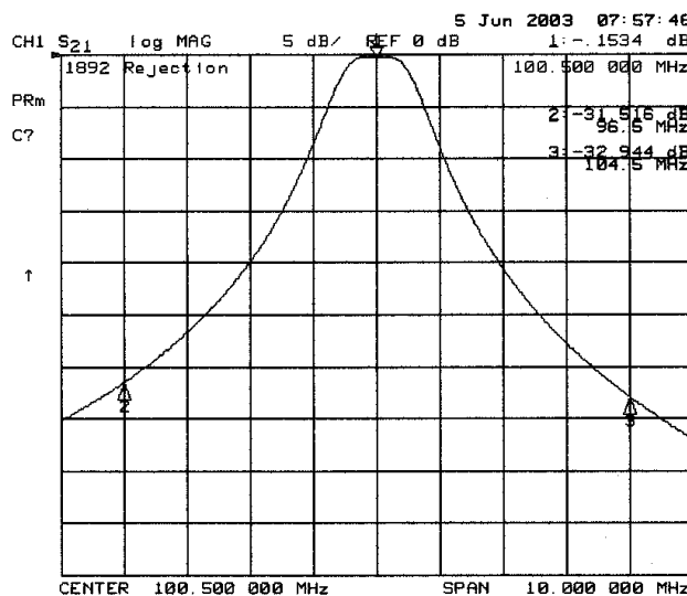
Rejection Plot 2-section filter
